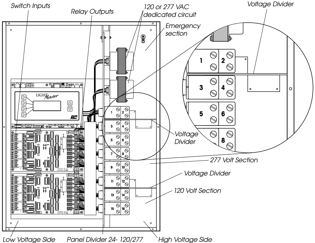
LightMaster 16 Relay Panel
