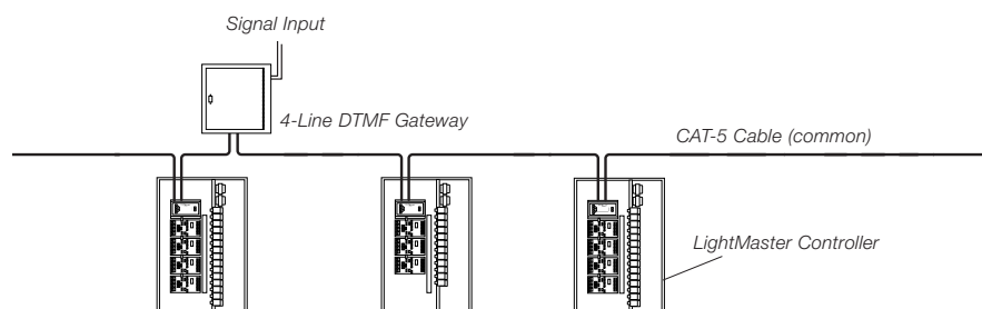
4-Line DTMF Gateway Connection to LightMaster network
