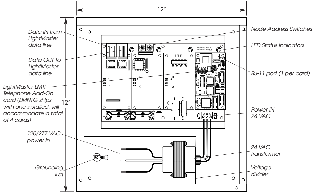
LightMaster 4-line DTMF Gateway (shown in NEMA-type enclosure with transformer)
