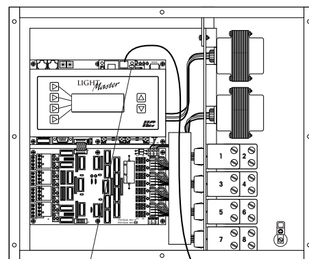
DTMF Card installed in Expansion Slot (under Keypad/Display)
